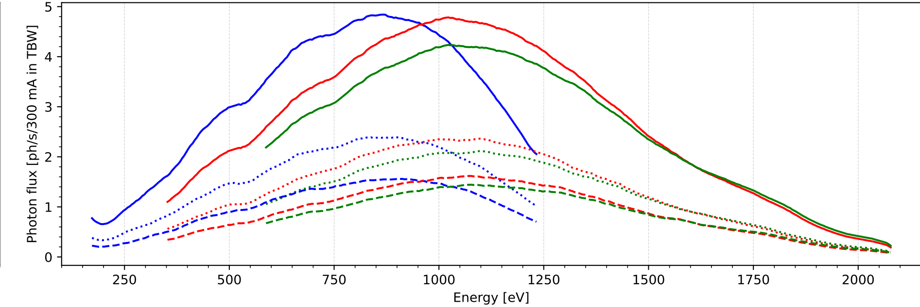
Flux Density on Sample
